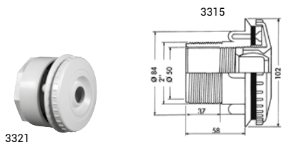
2" - 50 mm Cofies multi-directional outlet for Vinyl and Panel pools
