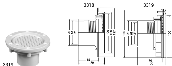
2" screw-in and 63 mm Cofies adjustable outlet for Concrete and Vinyl pools
