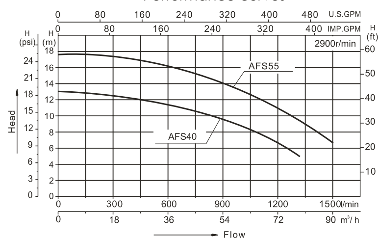
Performance curves
