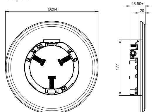
Faceplate
