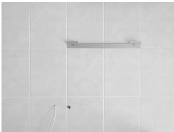
An example of preparation of electric power supply, condensate drainage and mounting of the bracket
